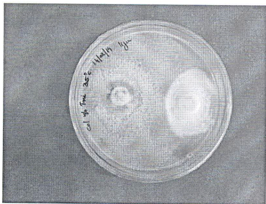
Fig. 3: Antagonistic test between T. viride (green colonies) and C. alienum
