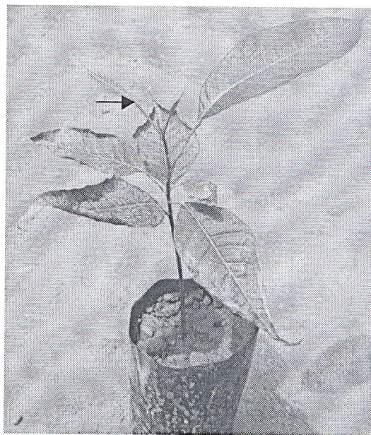
Fig. 5: S. macrophylla seedling showing recovery from the disease due to T. viride : Arrow mark indicates sprouting of new leaves
