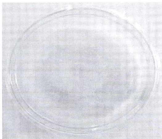
Fig. 1: C. alienum colony in PDA medium
